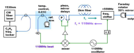
Figure 1: Schematic setup of the setup of the frequency domain stabilization scheme.[7]
