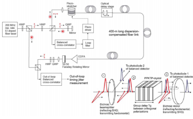
Figure 5: Experimental setup of the fiber link stabilization. lower right: Principle of the balanced optical cross-correlator [14].
