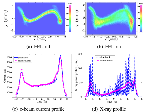
Figure 3: The simulated images on the screen representing e-beam longitudinal phase space for FEL-off (a) and FEL-on (b). The bunch charge is 250 \text{ pC} with an energy of 13.6 \text{ GeV} . (c) and (d) show the reconstructed e-beam current and FEL X-ray profiles comparing with the simulated ones. Bunch head is to the left.
