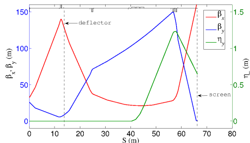
Figure 2: The optics layout for this diagnostics. The locations of the deflector and screen are marked in the picture.
